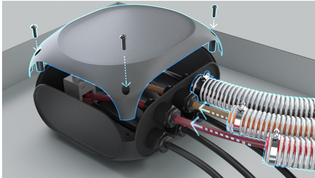
5. Mount the conduit pipes The cables need to be placed in separate conduit pipes and close the connection box.
