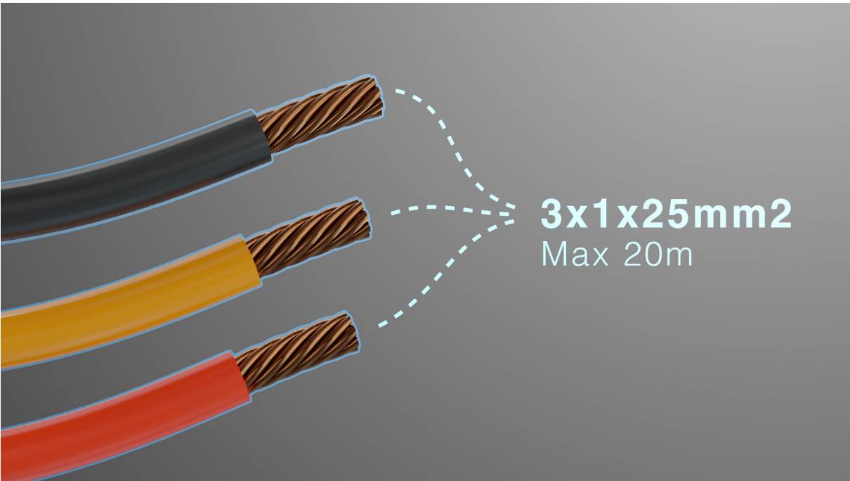
2. Choose your cable Use 3x1x25mm2 cable to a maximum cable length of 20 meter (total maximal 25 meter inclusive existing cable).
